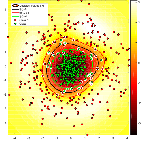
(b) \nu=0.09, \sigma=1.23, \text{SV}=52, \text{ACC}=0.97
