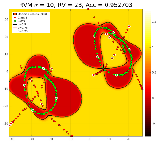
(c) RVM Decision Boundary
